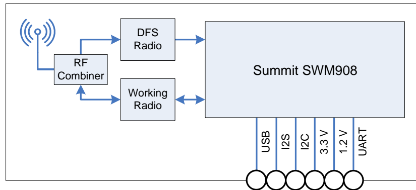
Summit SWM908SD TX Module Block Diagram
